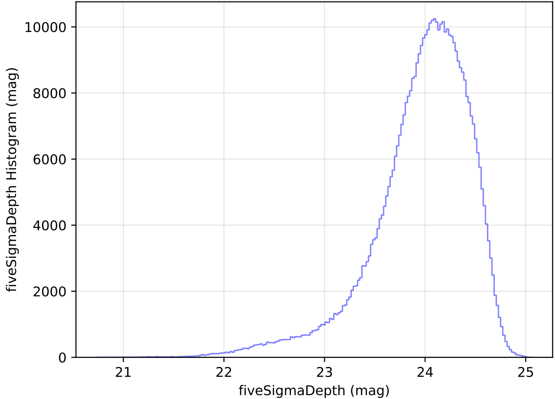
too_elab_heavy_r128_d2_ugrizy_v3.4_10yrs WFD r band: fiveSigmaDepth Histogram
