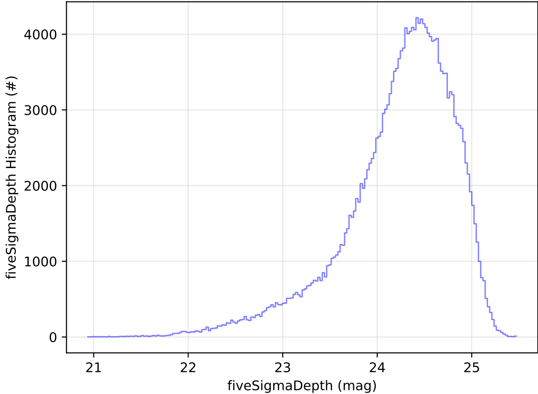
too_elab_heavy_r128_d2_ugrizy_v3.4_10yrs WFD g band: fiveSigmaDepth Histogram
