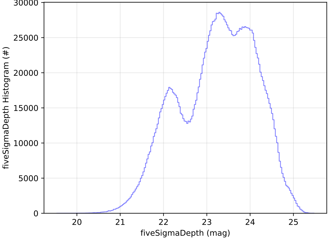
too_elab_heavy_r128_d2_ugrizy_v3.4_10yrs WFD all bands: fiveSigmaDepth Histogram
