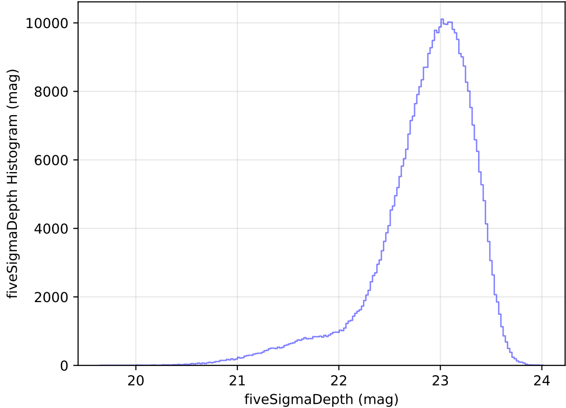
too_elab_heavy_r128_d2_ugrizy_v3.4_10yrs All sky z band: fiveSigmaDepth Histogram
