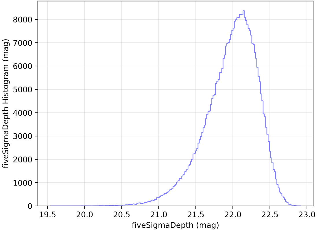
too_elab_heavy_r128_d2_ugrizy_v3.4_10yrs All sky y band: fiveSigmaDepth Histogram
