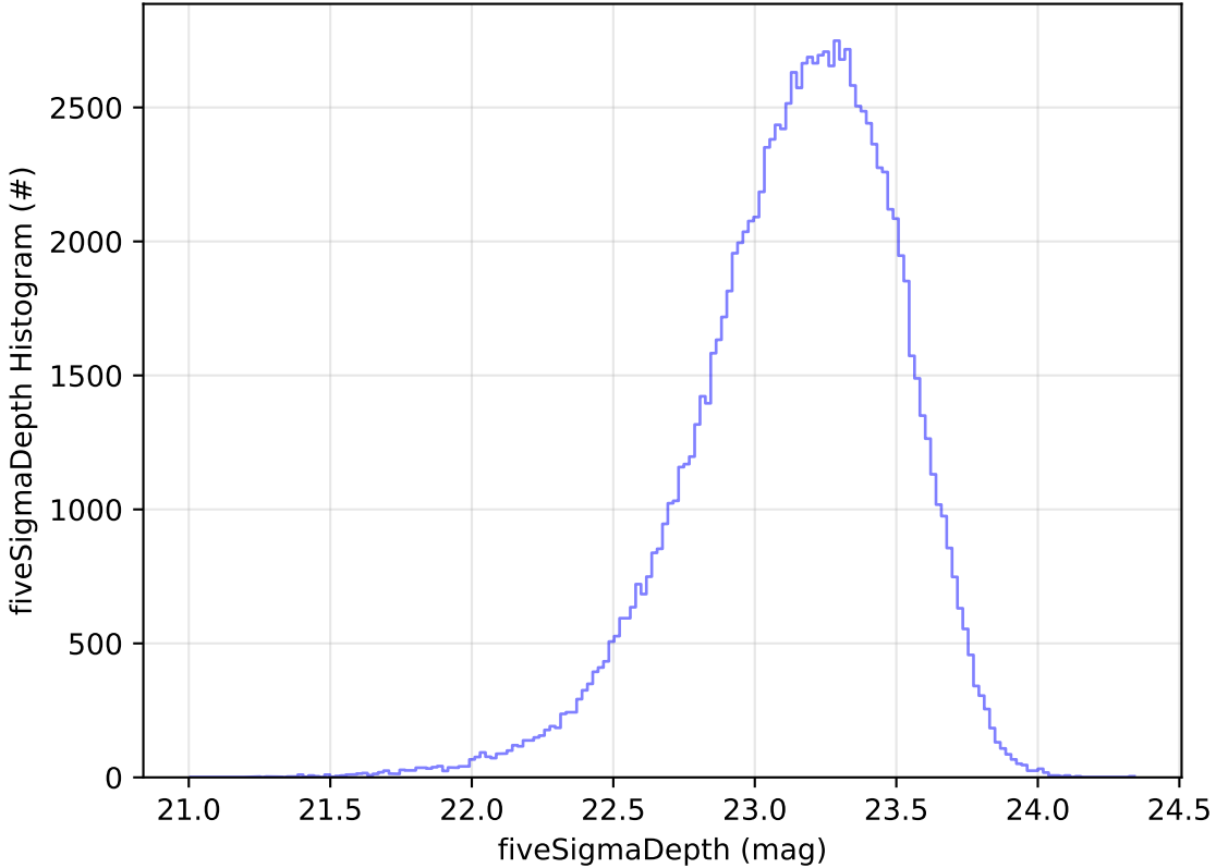
too_elab_heavy_r128_d2_ugrizy_v3.4_10yrs All sky u band: fiveSigmaDepth Histogram
