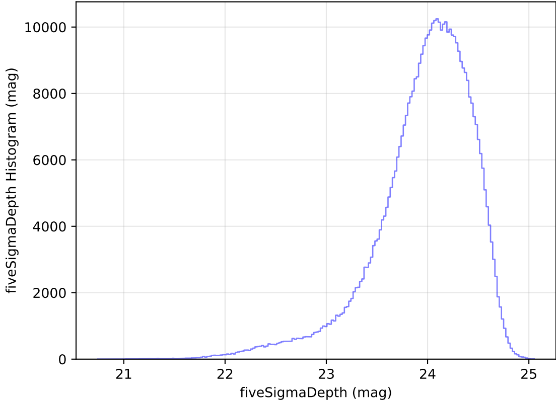
too_elab_heavy_r128_d2_ugrizy_v3.4_10yrs All sky r band: fiveSigmaDepth Histogram
