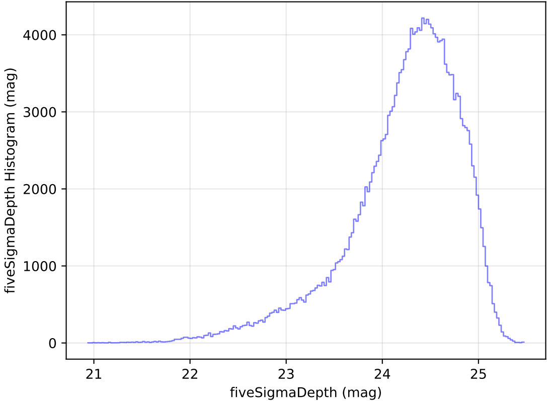
too_elab_heavy_r128_d2_ugrizy_v3.4_10yrs All sky g band: fiveSigmaDepth Histogram
