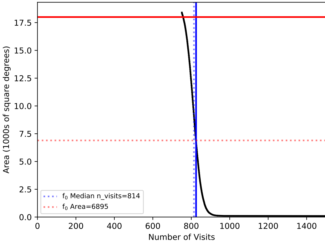
too_elab_heavy_r128_d2_ugrizy_v3.4_10yrs WFD: f0
