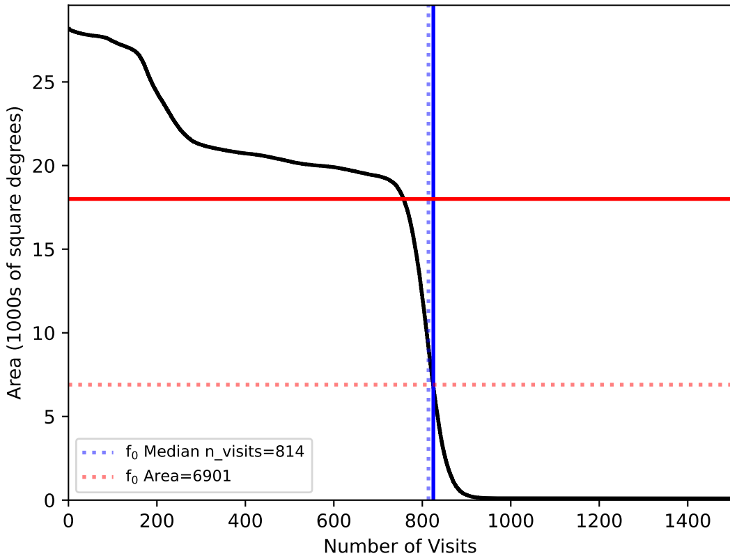
too_elab_heavy_r128_d2_ugrizy_v3.4_10yrs All sky: f0
