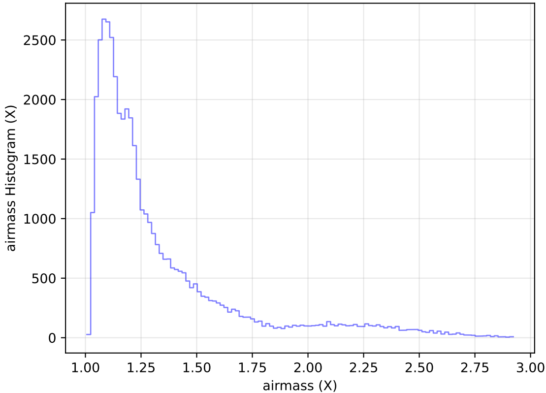
too_elab_heavy_r128_d2_ugrizy_v3.4_10yrs Yr 1 z band: airmass Histogram
