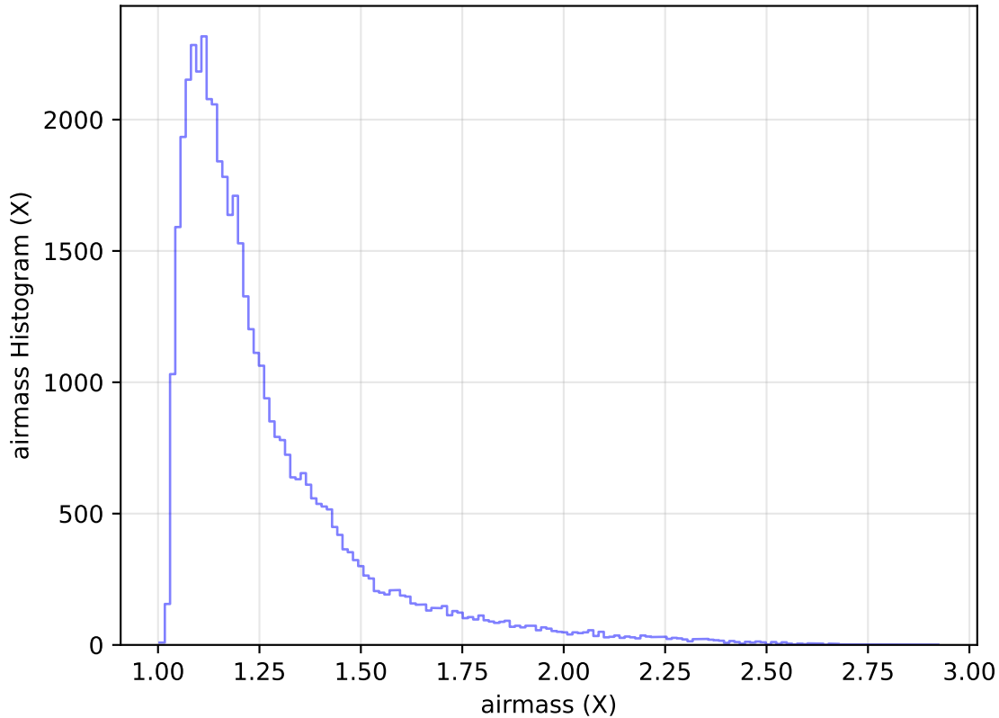
too_elab_heavy_r128_d2_ugrizy_v3.4_10yrs Yr 1 y band: airmass Histogram
