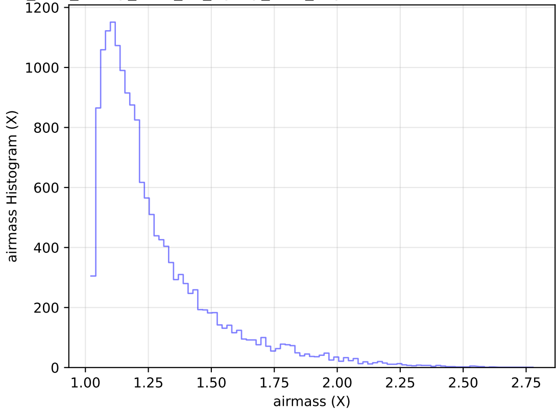
too_elab_heavy_r128_d2_ugrizy_v3.4_10yrs Yr 1 u band: airmass Histogram
