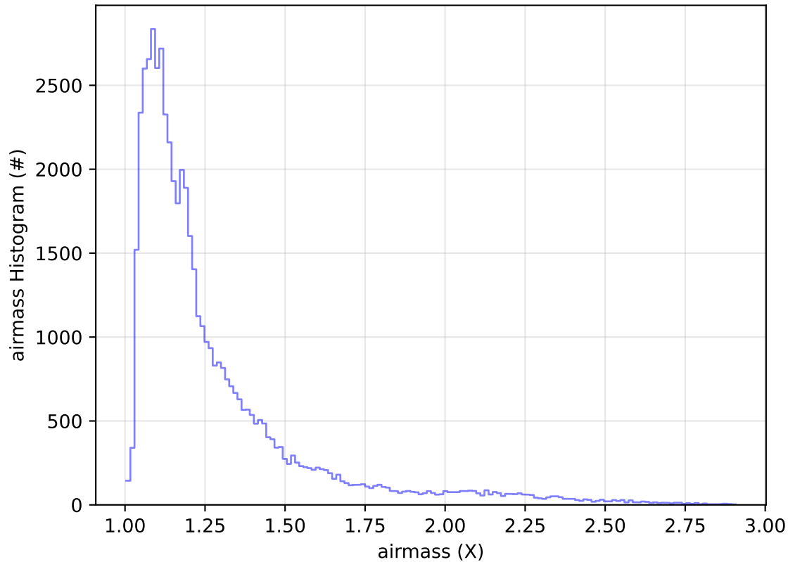
too_elab_heavy_r128_d2_ugrizy_v3.4_10yrs Yr 1 i band: airmass Histogram
