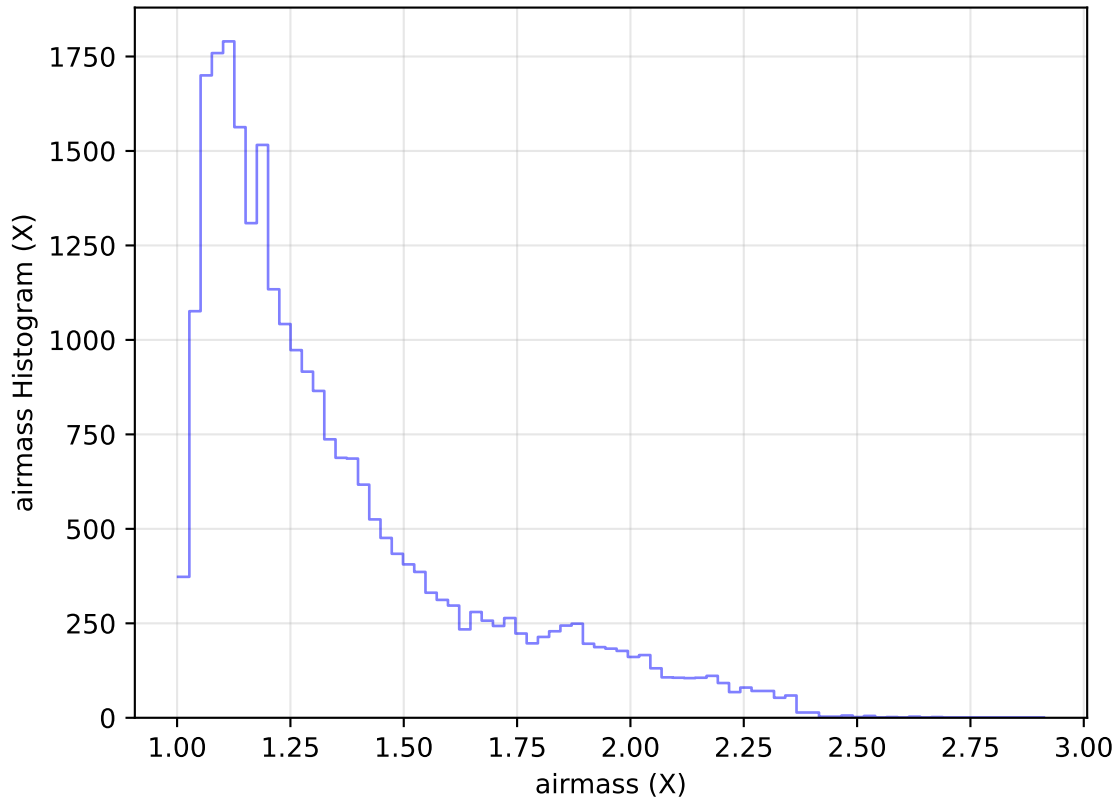
too_elab_heavy_r128_d2_ugrizy_v3.4_10yrs Yr 1 g band: airmass Histogram
