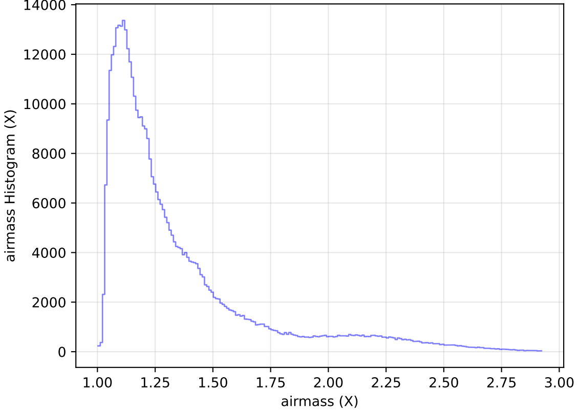
too_elab_heavy_r128_d2_ugrizy_v3.4_10yrs WFD z band: airmass Histogram
