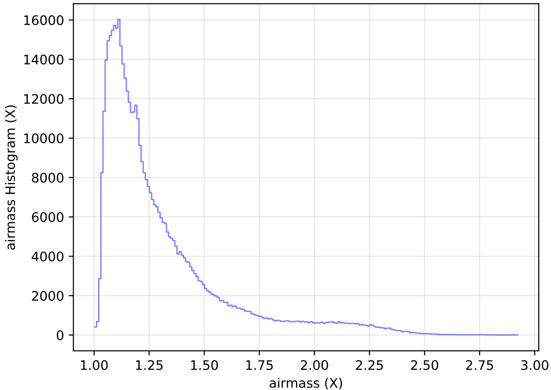
too_elab_heavy_r128_d2_ugrizy_v3.4_10yrs WFD r band: airmass Histogram
