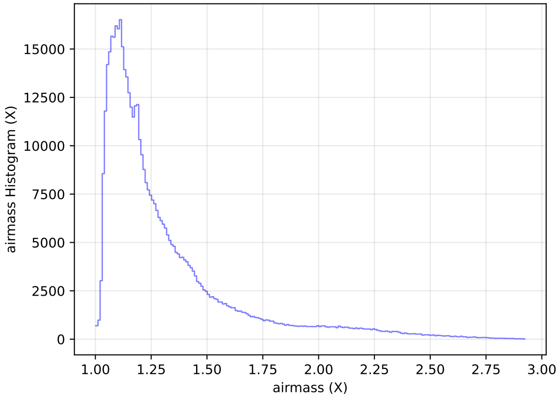
too_elab_heavy_r128_d2_ugrizy_v3.4_10yrs WFD i band: airmass Histogram
