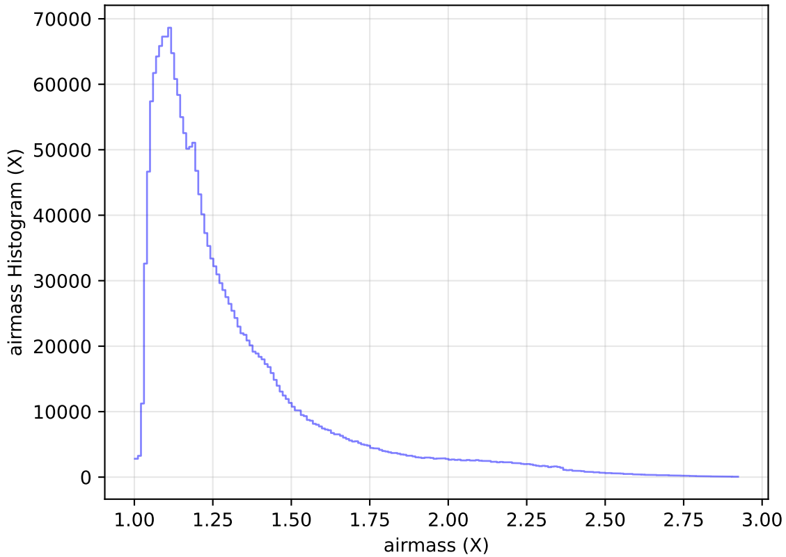
too_elab_heavy_r128_d2_ugrizy_v3.4_10yrs WFD all bands: airmass Histogram
