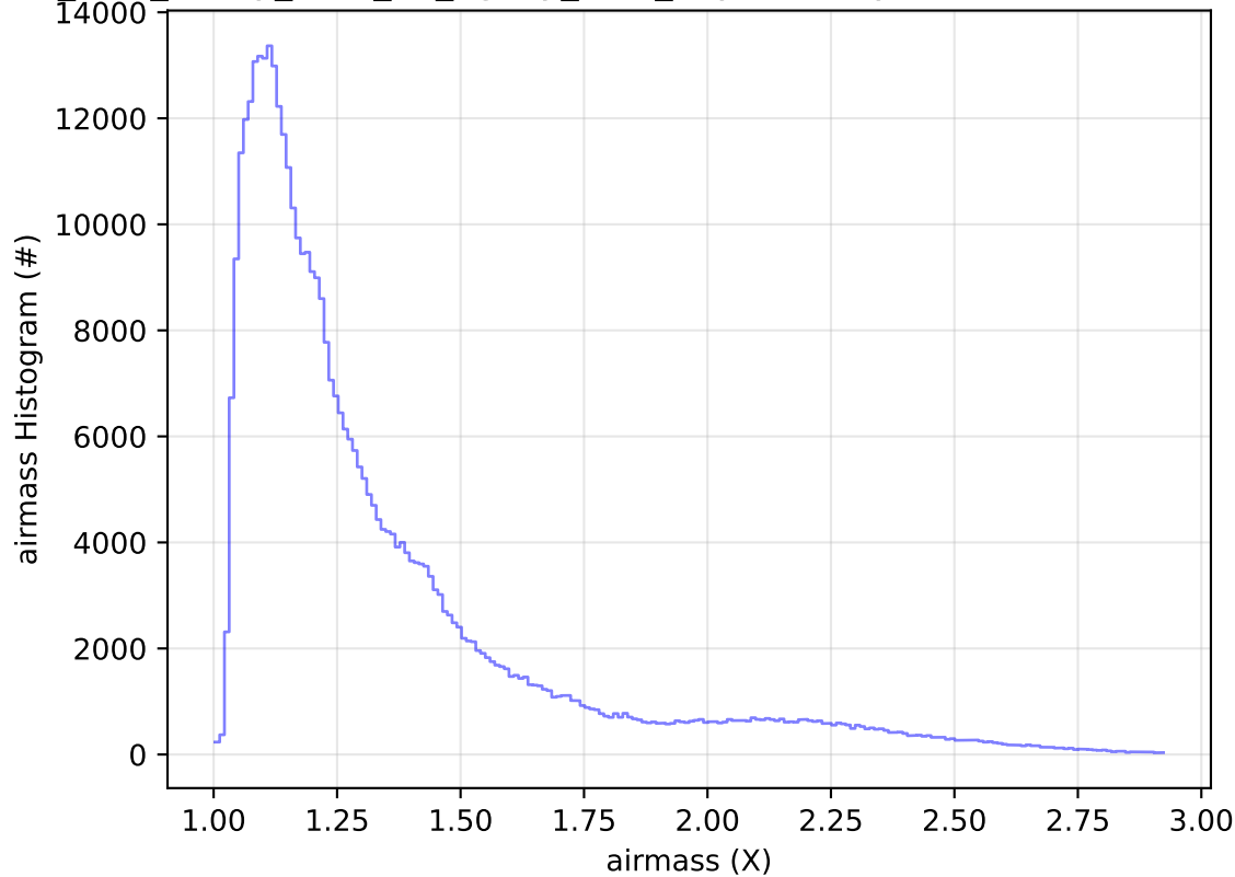
too_elab_heavy_r128_d2_ugrizy_v3.4_10yrs All sky z band: airmass Histogram
