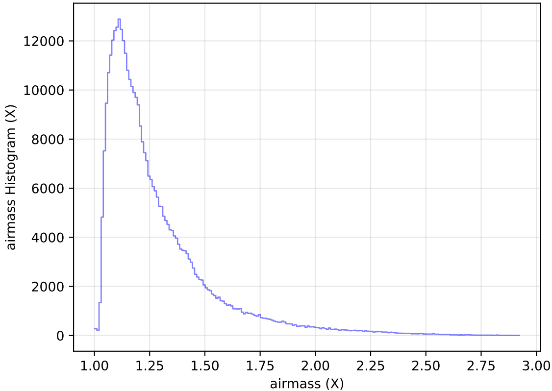
too_elab_heavy_r128_d2_ugrizy_v3.4_10yrs All sky y band: airmass Histogram
