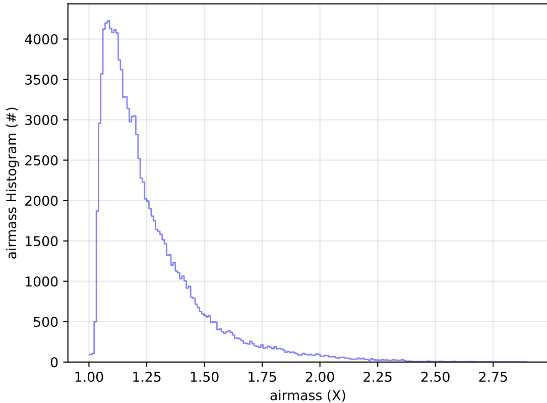
too_elab_heavy_r128_d2_ugrizy_v3.4_10yrs All sky u band: airmass Histogram
