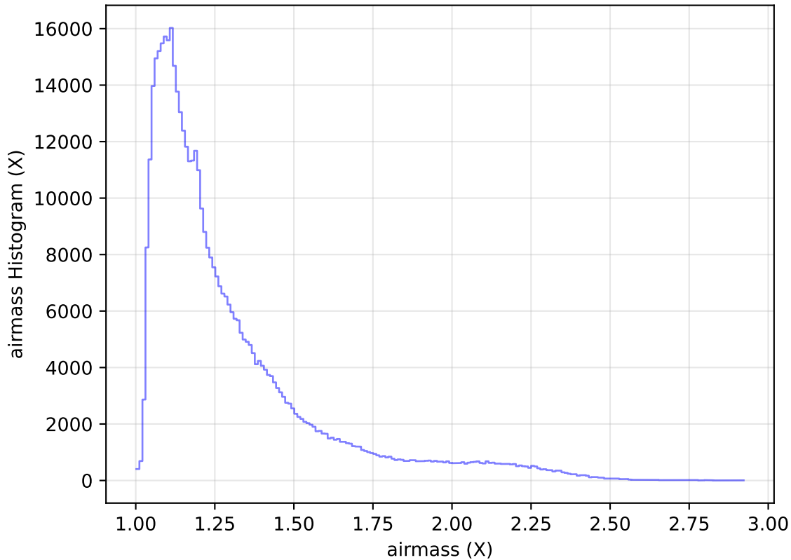
too_elab_heavy_r128_d2_ugrizy_v3.4_10yrs All sky r band: airmass Histogram
