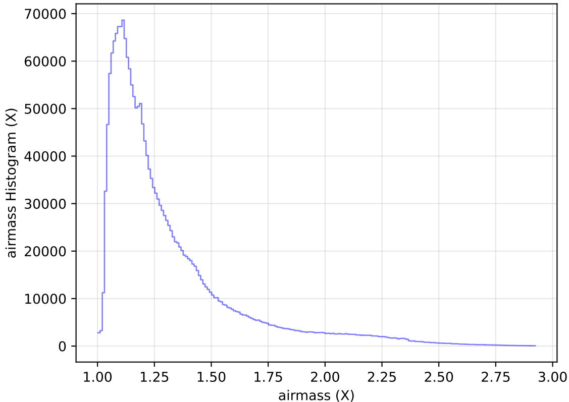
too_elab_heavy_r128_d2_ugrizy_v3.4_10yrs All sky all bands: airmass Histogram
