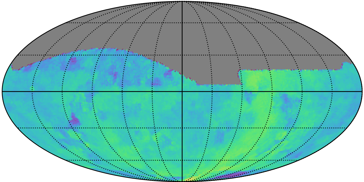
too_elab_heavy_r128_d2_ugrizy_v3.4_10yrs All sky: Parallax Coverage @ 24.0
