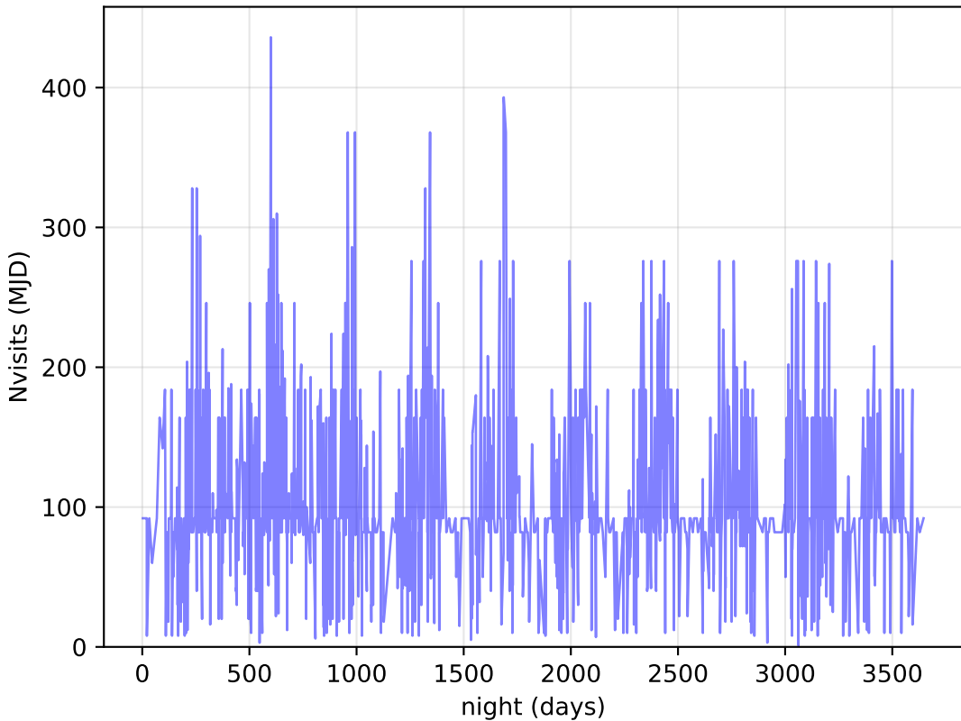
too_elab_heavy_r128_d2_ugrizy_v3.4_10yrs DDF: Nvisits
