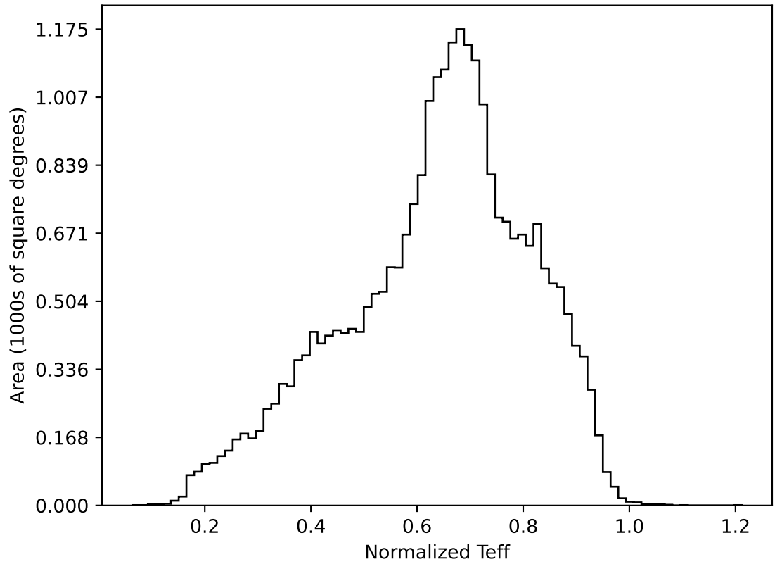
too_elab_heavy_r128_d2_ugrizy_v3.4_10yrs All sky all bands: Normalized Teff
