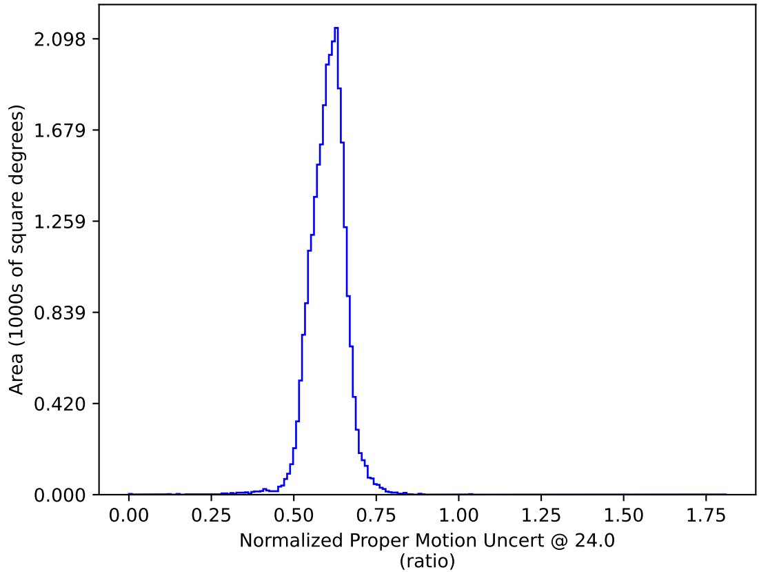
too_elab_heavy_r128_d2_ugrizy_v3.4_10yrs All sky: Normalized Proper Motion Uncert @ 24.0
