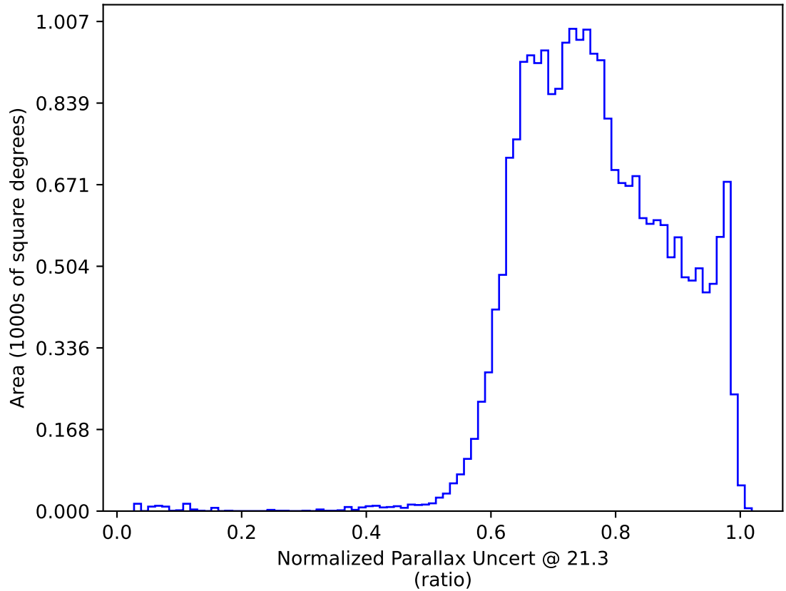
too_elab_heavy_r128_d2_ugrizy_v3.4_10yrs All sky y band only: Normalized Parallax Uncert @ 21.3
