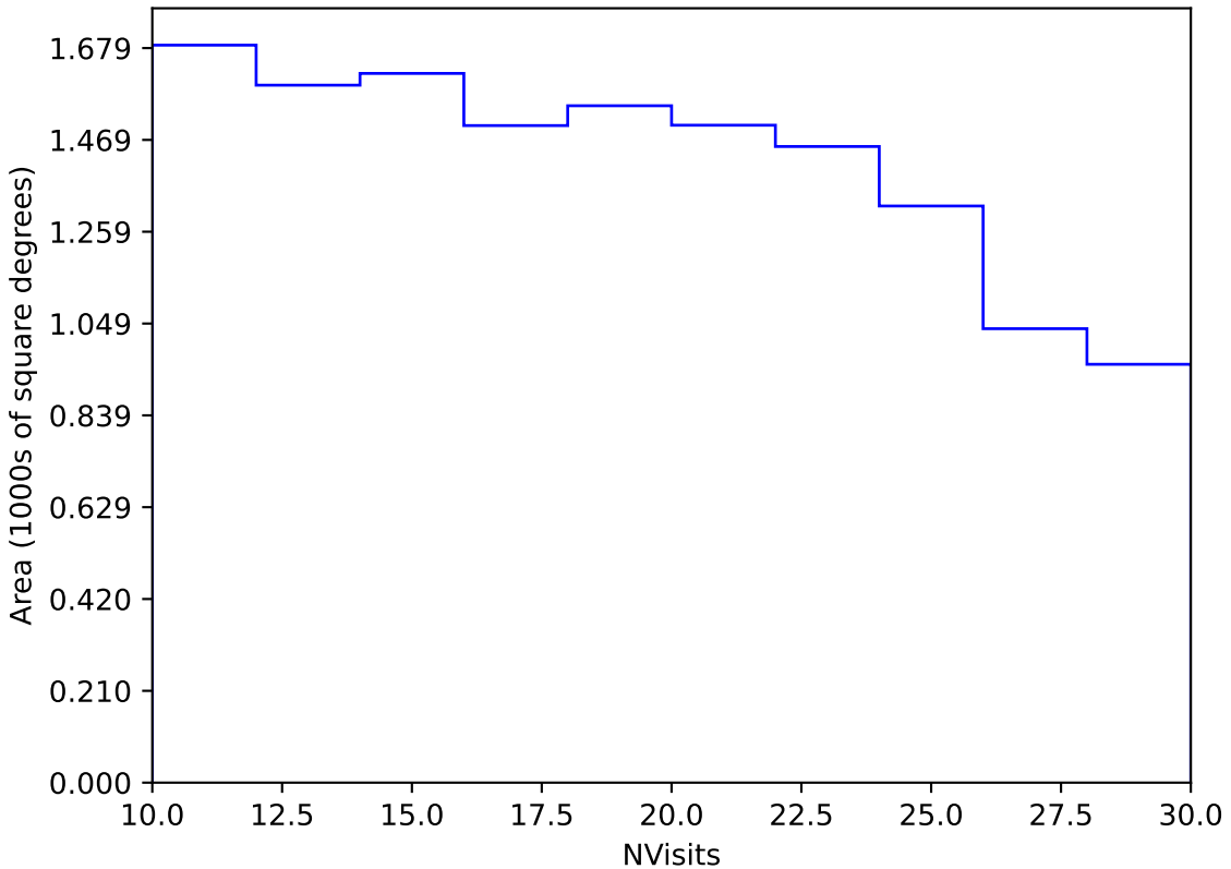
too_elab_heavy_r128_d2_ugrizy_v3.4_10yrs Yr 3-4 y band: NVisits
