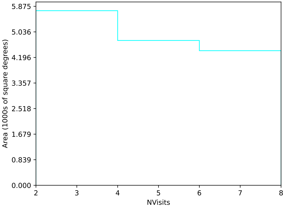
too_elab_heavy_r128_d2_ugrizy_v3.4_10yrs Yr 3-4 u band: NVisits
