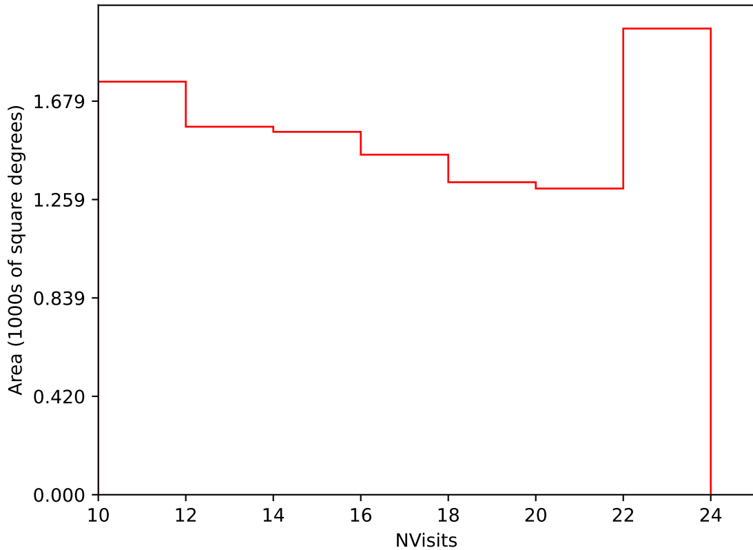
too_elab_heavy_r128_d2_ugrizy_v3.4_10yrs Yr 3-4 i band: NVisits
