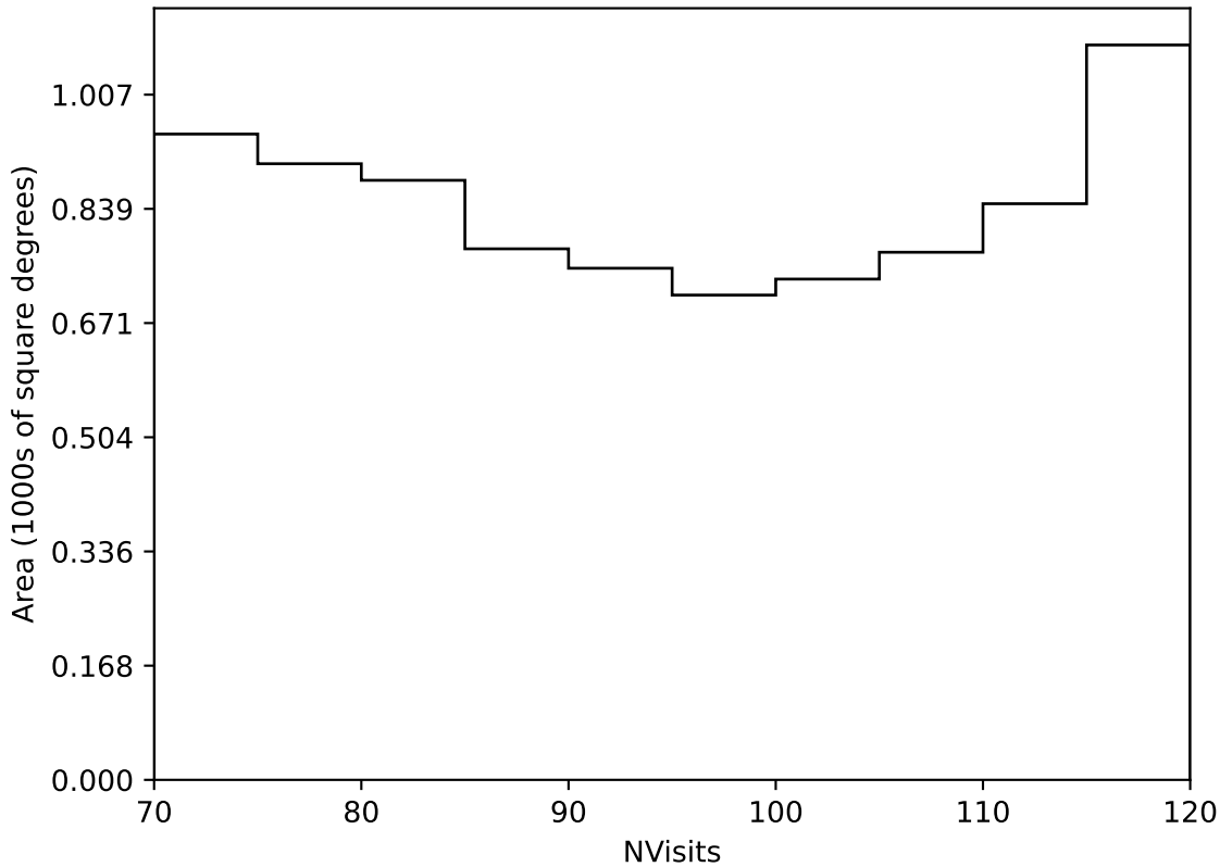
too_elab_heavy_r128_d2_ugrizy_v3.4_10yrs Yr 3-4 all bands: NVisits
