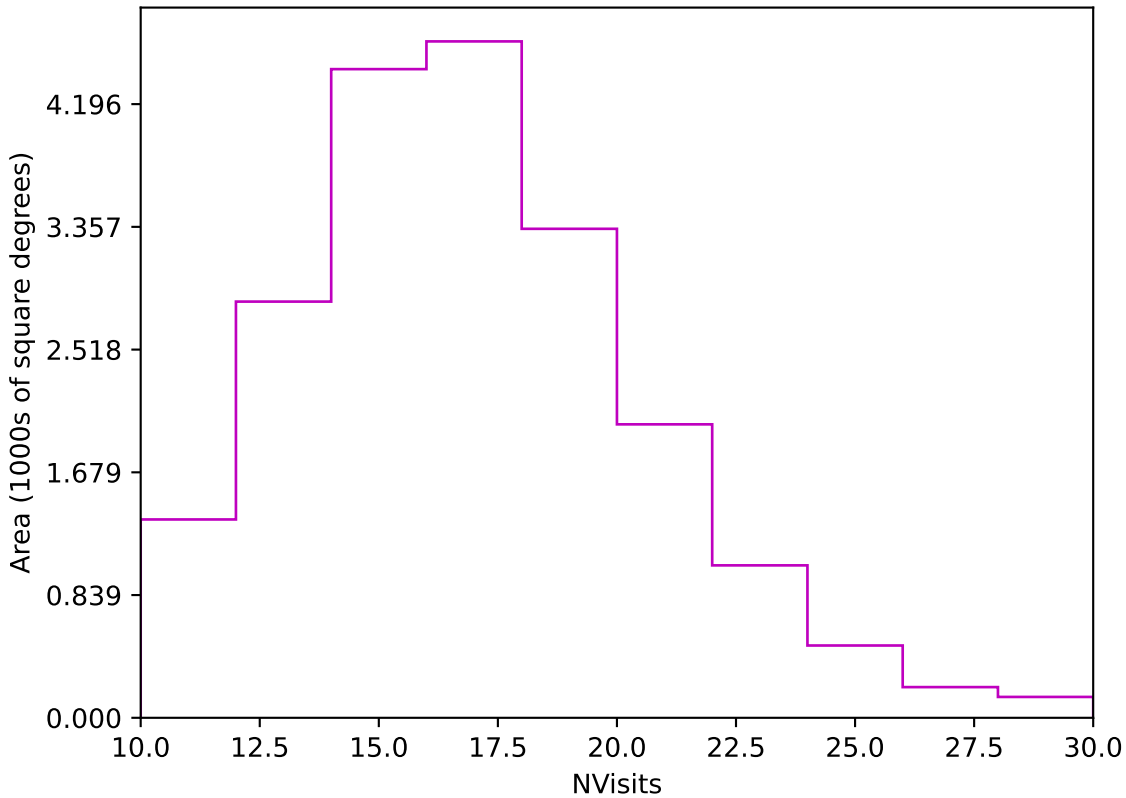
too_elab_heavy_r128_d2_ugrizy_v3.4_10yrs Yr 1 z band: NVisits
