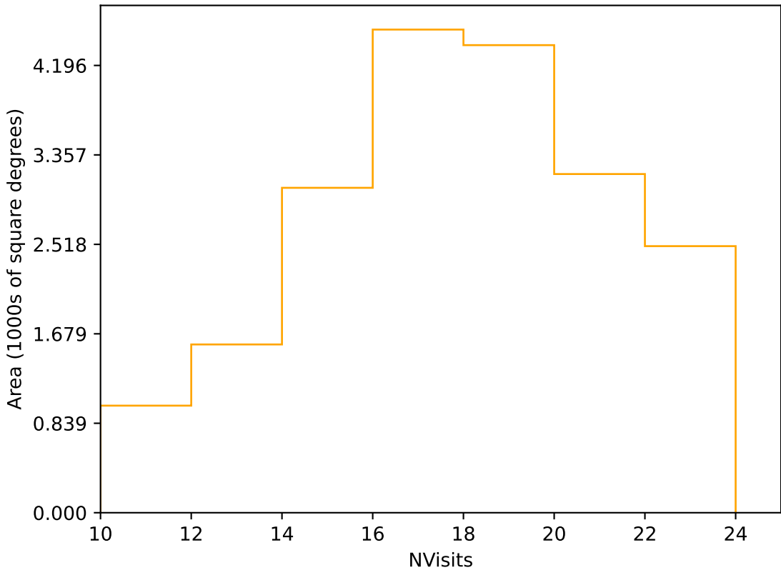
too_elab_heavy_r128_d2_ugrizy_v3.4_10yrs Yr 1 r band: NVisits
