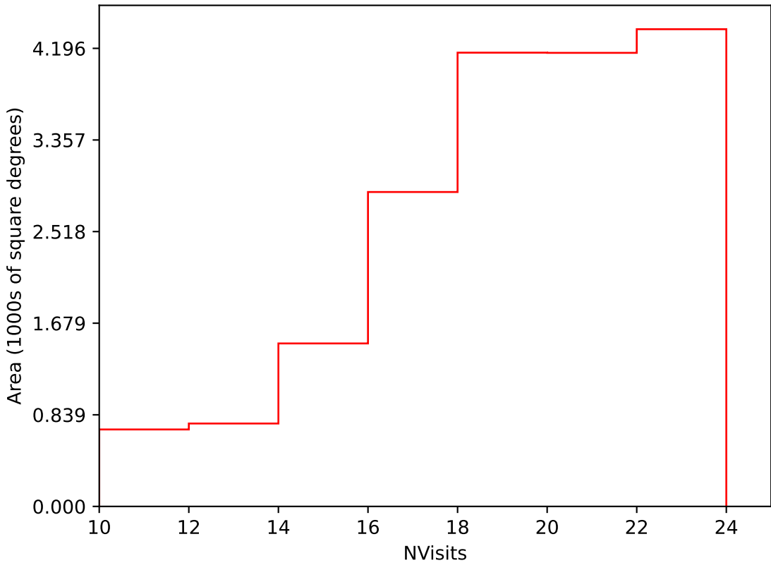
too_elab_heavy_r128_d2_ugrizy_v3.4_10yrs Yr 1 i band: NVisits
