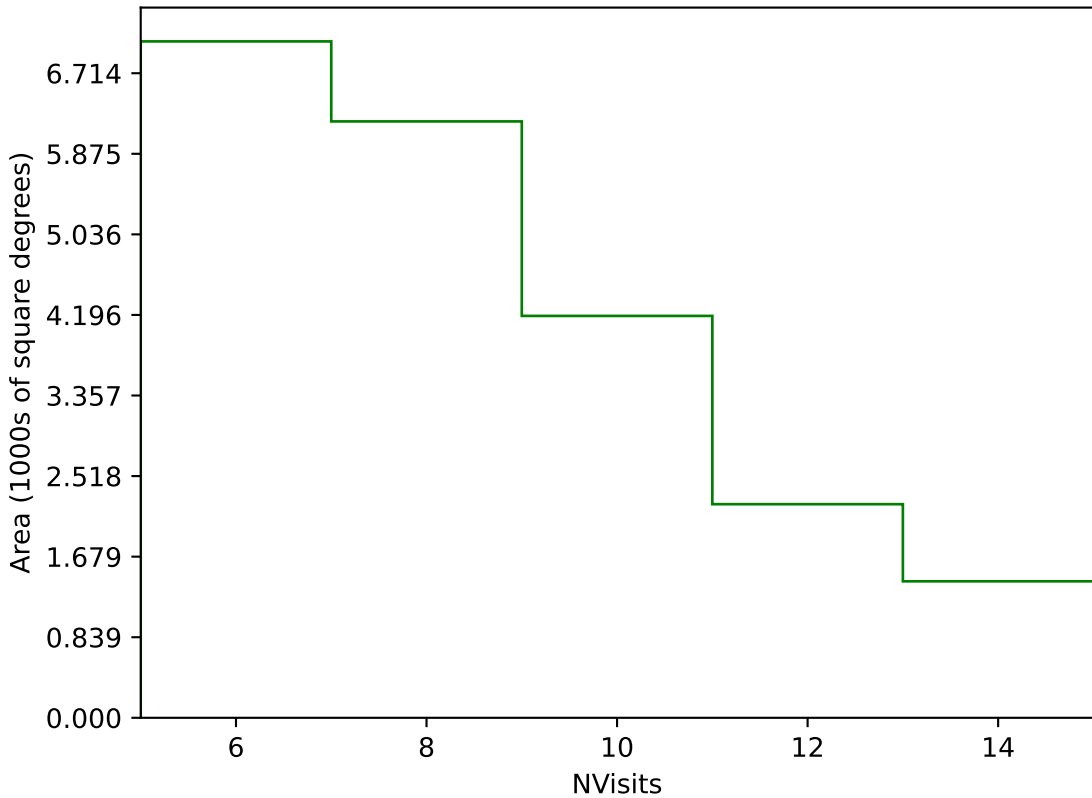
too_elab_heavy_r128_d2_ugrizy_v3.4_10yrs Yr 1 g band: NVisits
