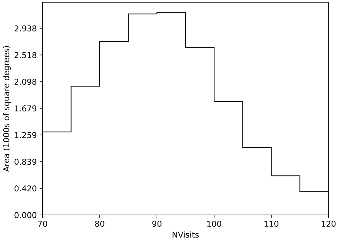
too_elab_heavy_r128_d2_ugrizy_v3.4_10yrs Yr 1 all bands: NVisits
