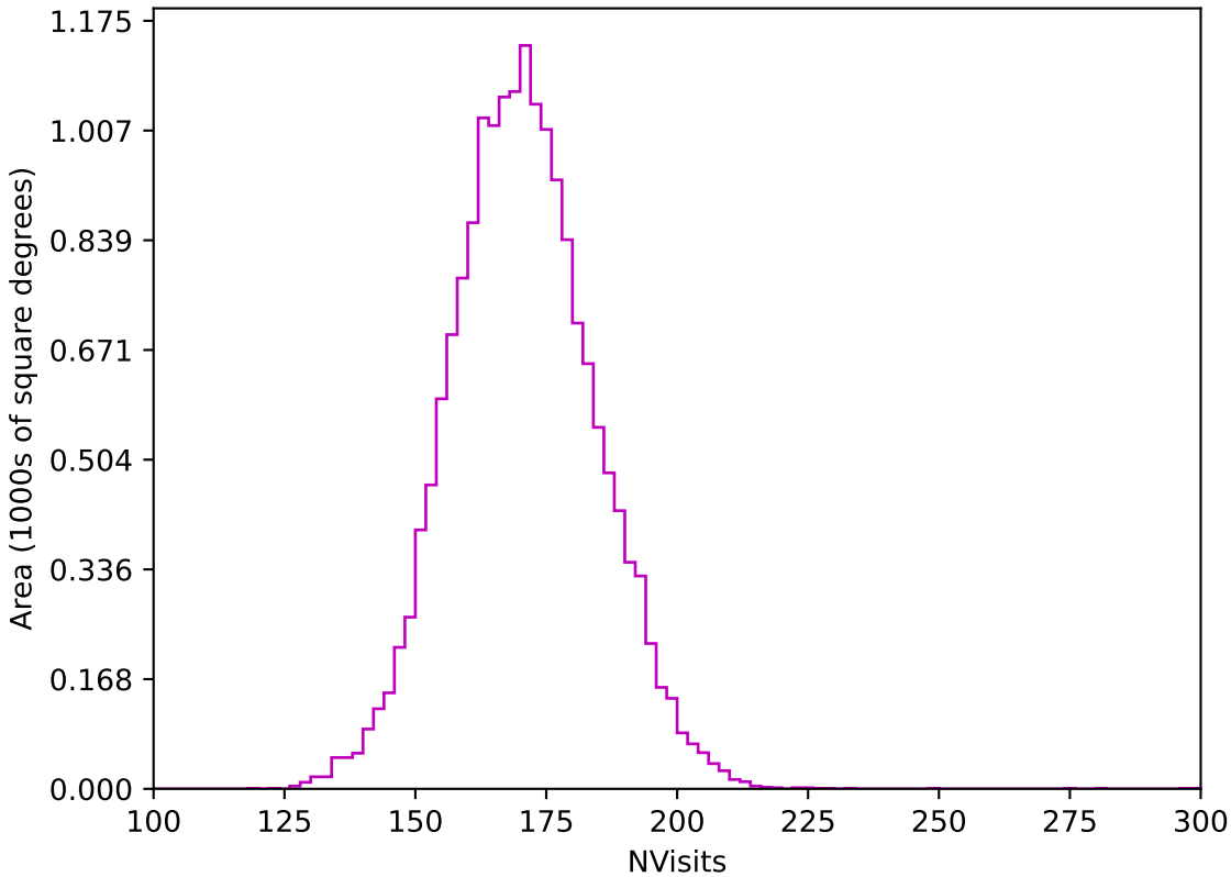
too_elab_heavy_r128_d2_ugrizy_v3.4_10yrs WFD z band: NVisits
