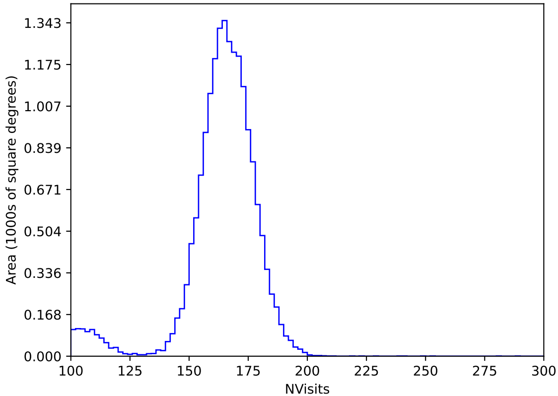
too_elab_heavy_r128_d2_ugrizy_v3.4_10yrs WFD y band: NVisits
