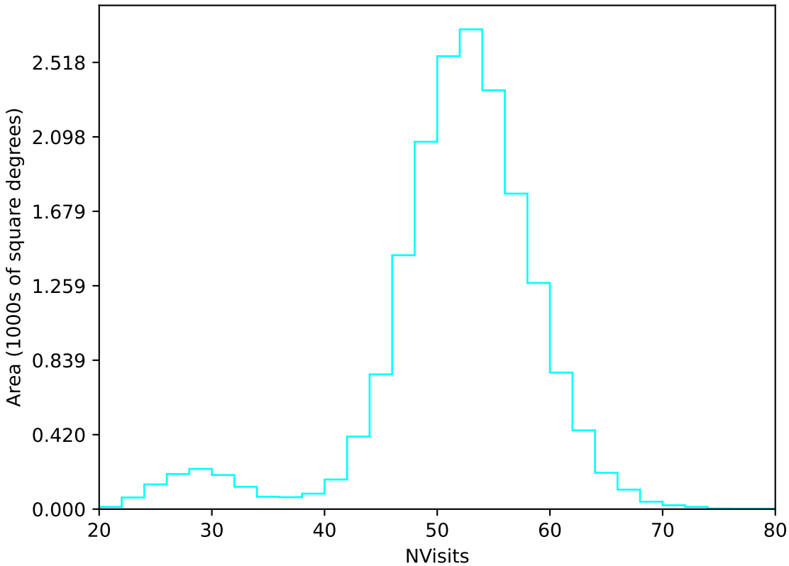
too_elab_heavy_r128_d2_ugrizy_v3.4_10yrs WFD u band: NVisits
