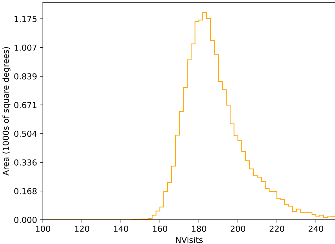
too_elab_heavy_r128_d2_ugrizy_v3.4_10yrs WFD r band: NVisits
