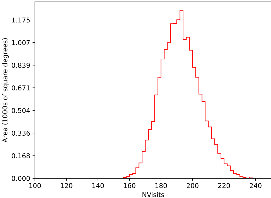
too_elab_heavy_r128_d2_ugrizy_v3.4_10yrs WFD i band: NVisits
