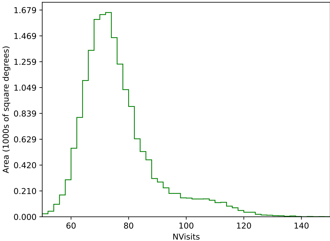
too_elab_heavy_r128_d2_ugrizy_v3.4_10yrs WFD g band: NVisits
