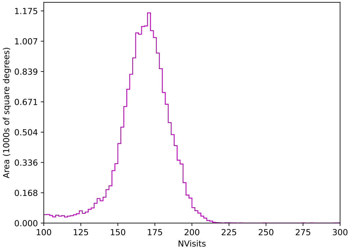
too_elab_heavy_r128_d2_ugrizy_v3.4_10yrs All sky z band: NVisits
