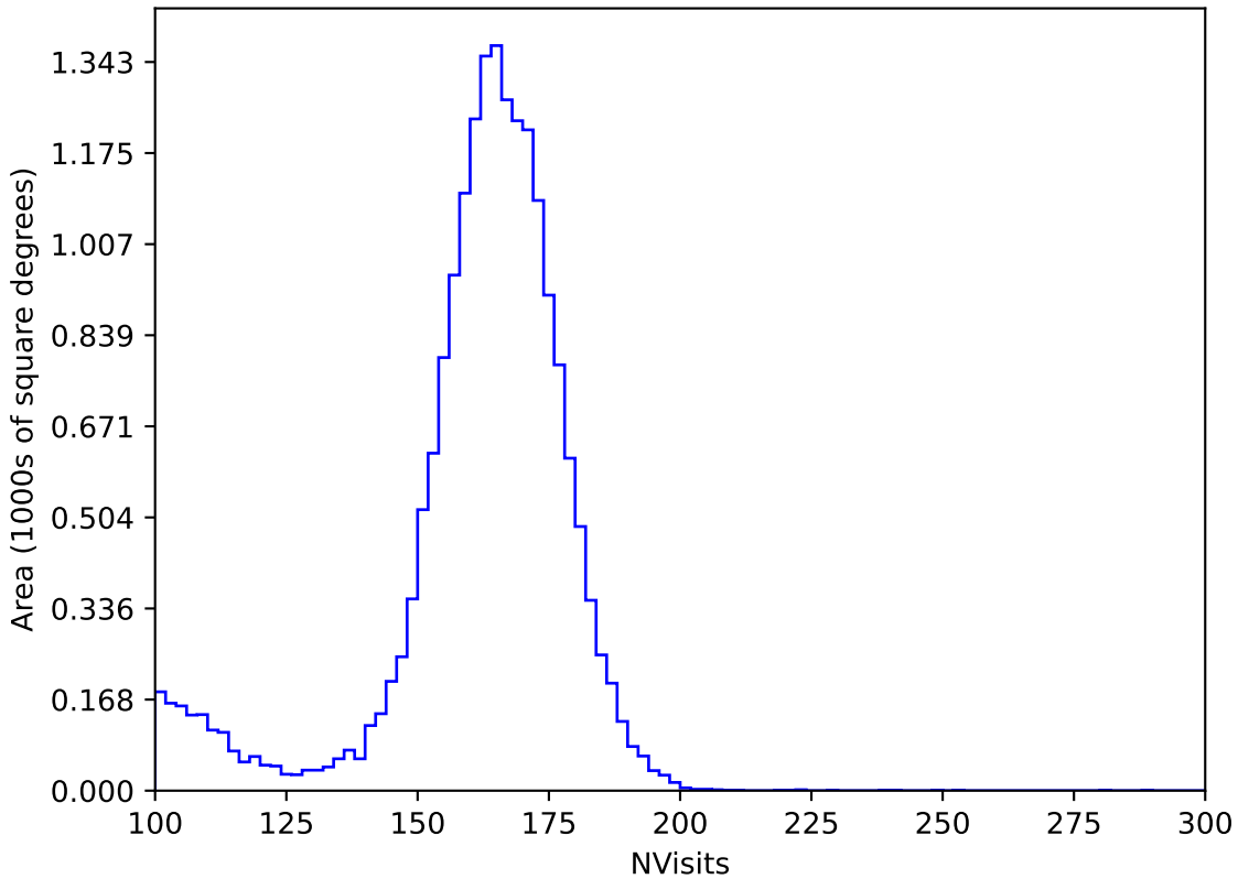
too_elab_heavy_r128_d2_ugrizy_v3.4_10yrs All sky y band: NVisits
