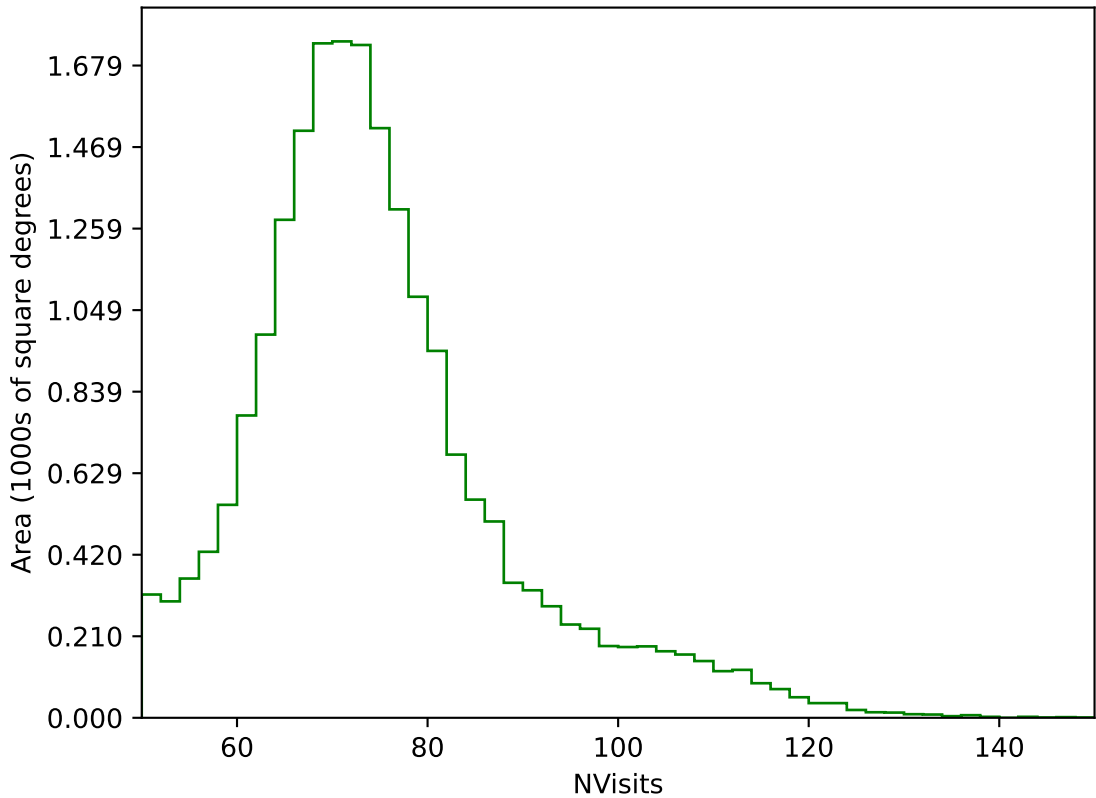
too_elab_heavy_r128_d2_ugrizy_v3.4_10yrs All sky g band: NVisits
