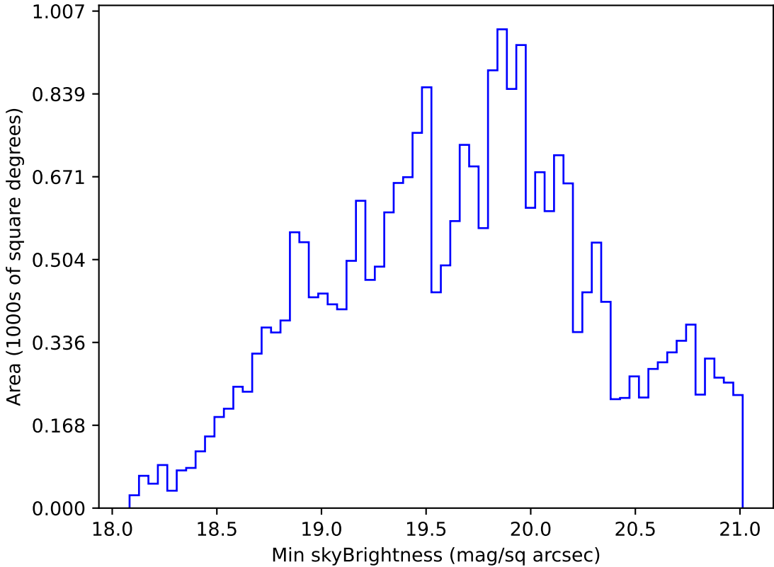
too_elab_heavy_r128_d2_ugrizy_v3.4_10yrs Yr 1 r band: Min skyBrightness
