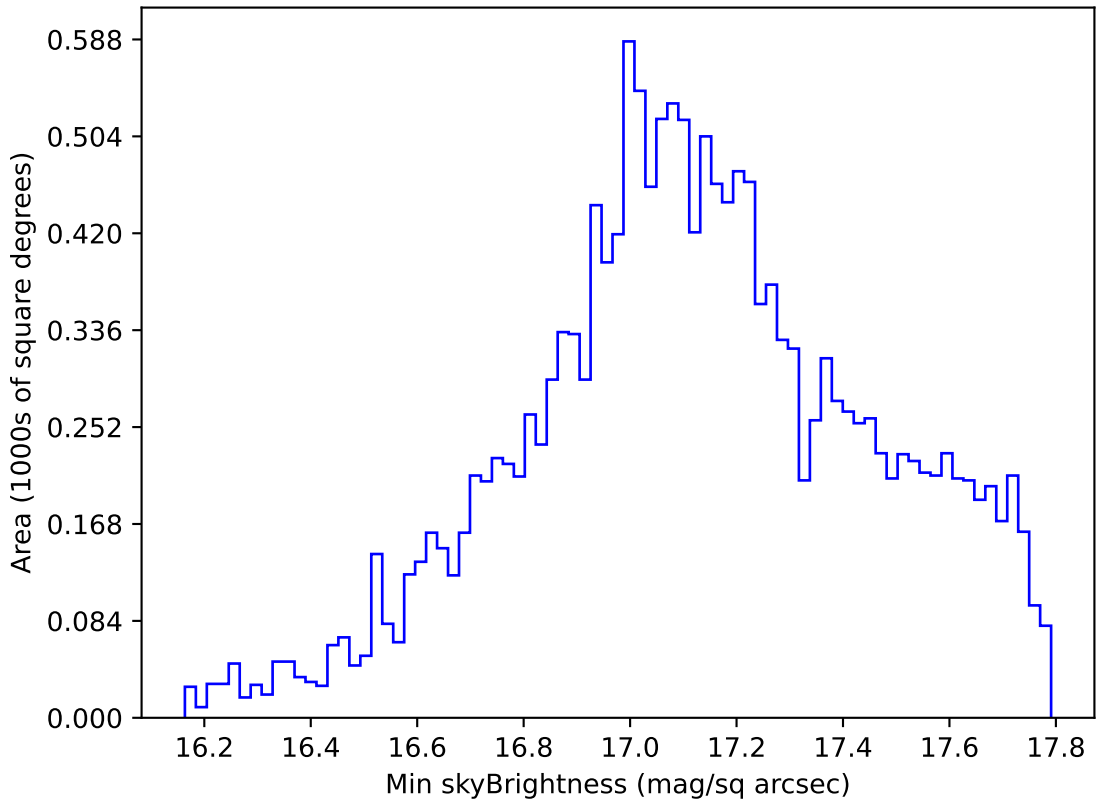
too_elab_heavy_r128_d2_ugrizy_v3.4_10yrs WFD y band: Min skyBrightness
