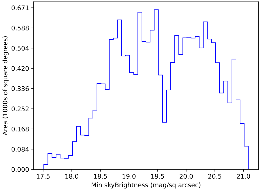
too_elab_heavy_r128_d2_ugrizy_v3.4_10yrs WFD g band: Min skyBrightness
